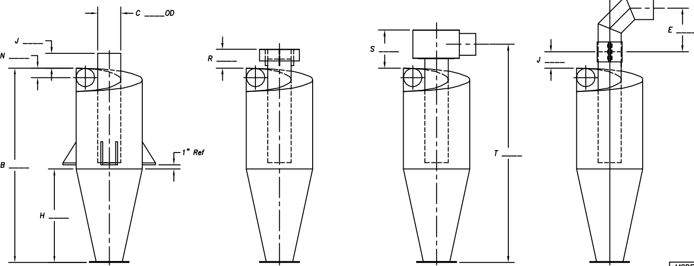
TYPE 1 AIR OUTLET TYPE 2 AIR OUTLET (RAIN SHIELD) TYPE 3 AIR OUTLET (LOW PROFILE OUTLET) (INFINITE OUTLET ORIENTATION) TYPE 4 AIR OUTLET
