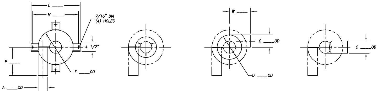
TYPE 1 AIR OUTLET TYPE 2 AIR OUTLET (RAIN SHIELD) TYPE 3 AIR OUTLET (LOW PROFILE OUTLET) (INFINITE OUTLET ORIENTATION) TYPE 4 AIR OUTLET
